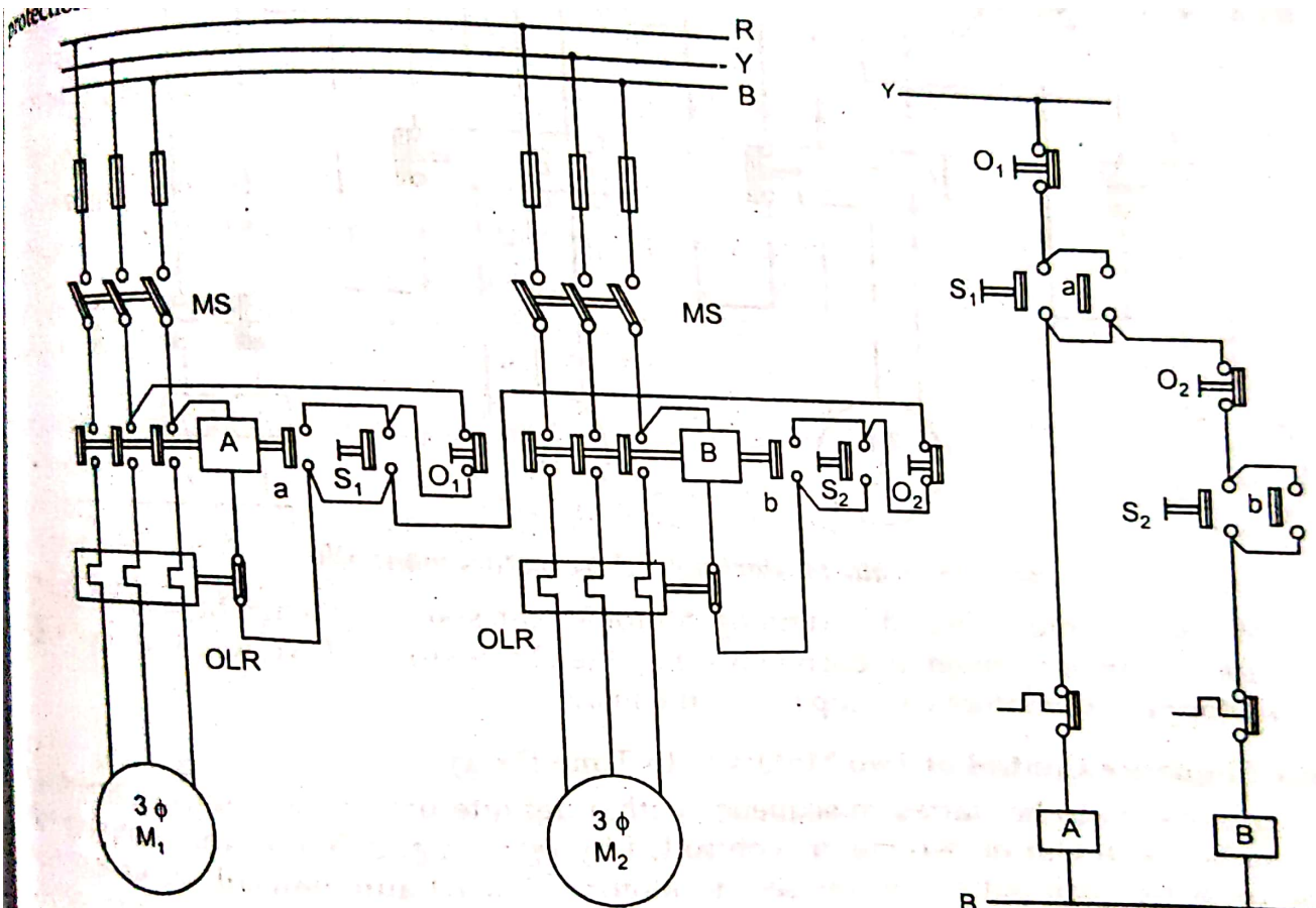
Fig. 7.25. Sequence starting of two motors manually
