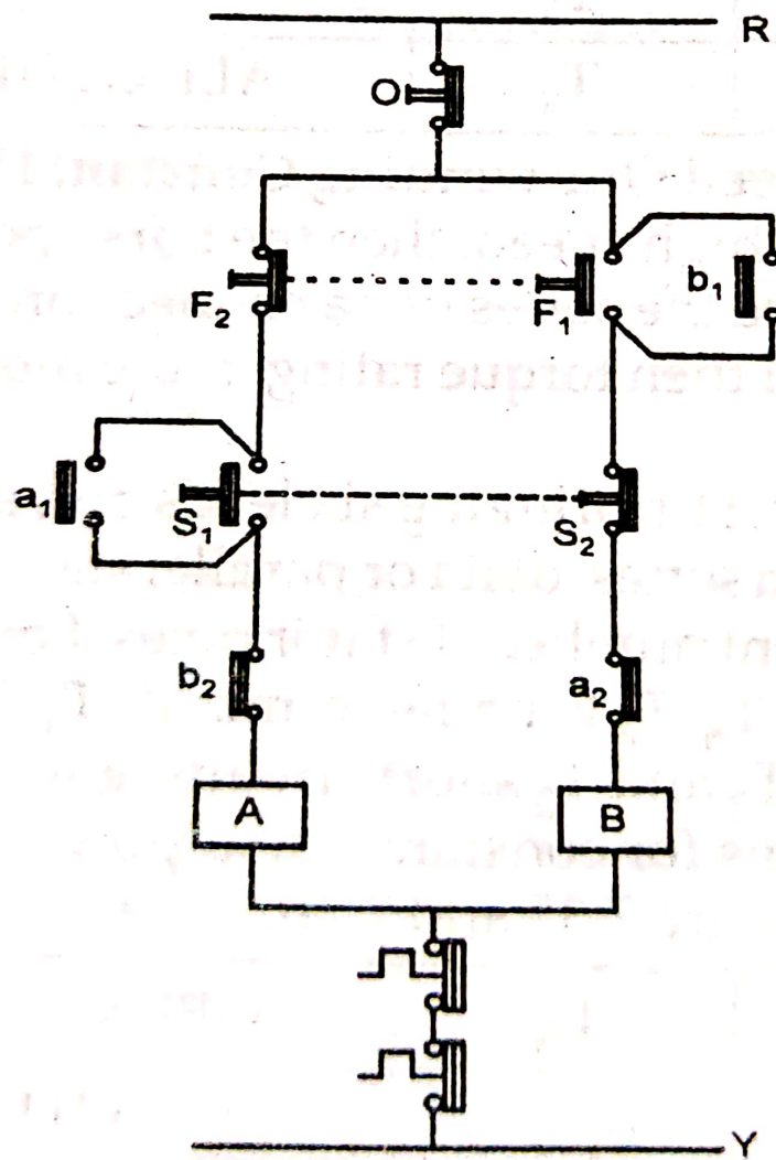
Fig. 7.37. 2 Speed induction motor control using INO + INC Push
