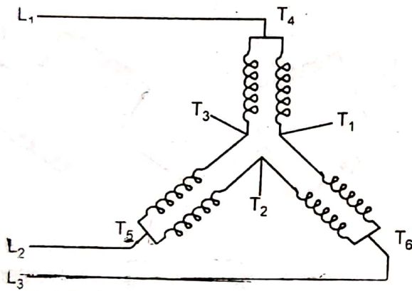
Fig. 7.35. Constant Torque Three phase squirrel cage motor connection arrangement for 2 speed one winding connection for constant torque.
