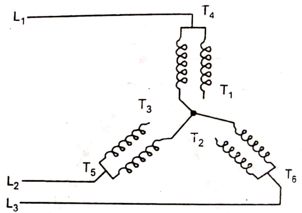
Fig. 7.36. Variable Torque Three phase two speedsquirrel cage connection arrangement for variable torque one stator winding
