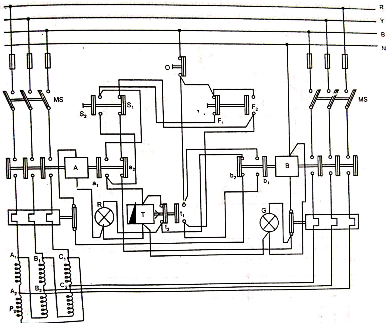
Fig. 7. 40. Automatic Two speed Motor Control. The three phase induction motor stator is wound for single winding two speed for constant horse power and constant torque.
