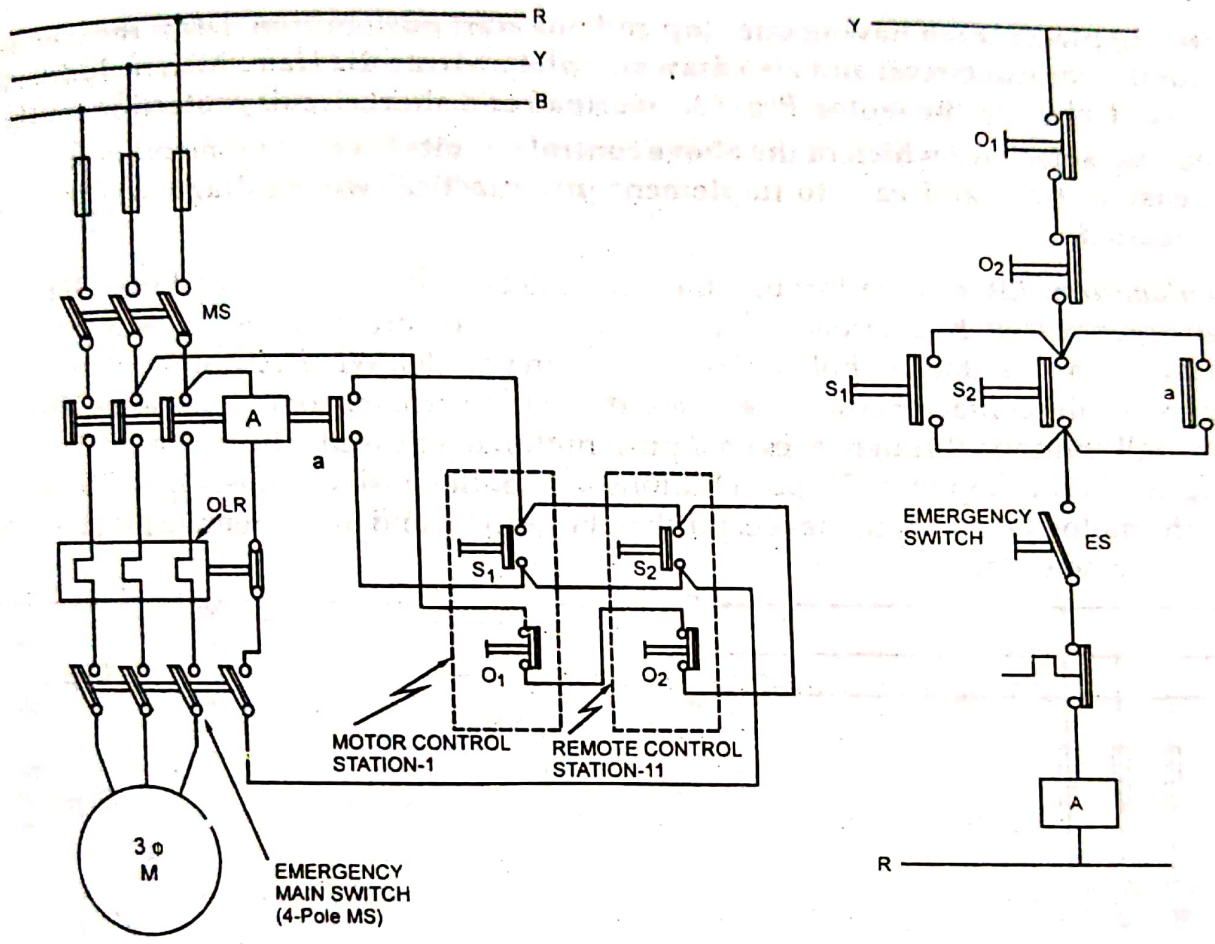
Motor Controlled From Two Locations. O 2 and S 2 are installed at a remote place for second alternate control.
